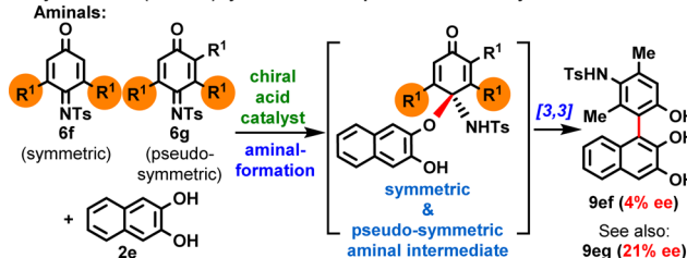
Figure 3. Symmetries of intermediates in chirality transfer processes have a dramatic impact on the final products' ee.
